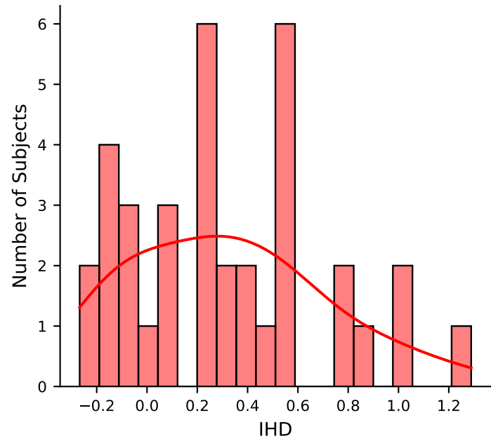
IHD Distribution
